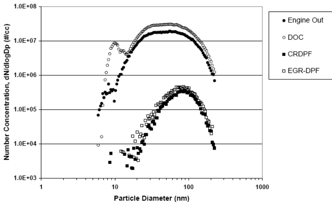
Figure 5. “CRDPF” is an engine equipped with a CRT and “EGR-DPF” is an engine with a CRT using exhaust gas recirculation. The CRT engines had lower UFP numbers across all particle sizes than the diesel engine with no controls and the engine with a diesel oxidation catalyst only (no trap). The test method used a minidiluter (Frank et al., 2006).
