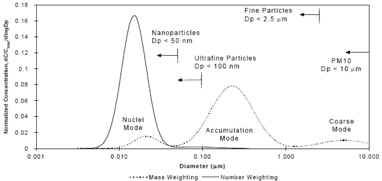
Figure 1. Idealized mass weighted (dashed line) and number weighted (solid line) distributions of particulate matter in diesel engine exhaust (Kittelson, 1998).
