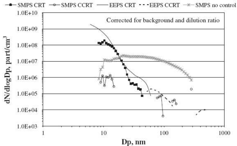
Figure 2. SMPS and EEPS size distributions for the CRT, CCRT, and uncontrolled case. SMPS and EEPS refer to different PM measurement methods. Note that the SMPS method substantially undercounts particles <0.01 \mu\text{m} (10 nm) in size relative to the EEPS method. The figure indicates the CRT produces higher UFP number than the CCRT and the uncontrolled engine. The CCRT produces the lowest UFP number (Kittelson et al., 2006a).
