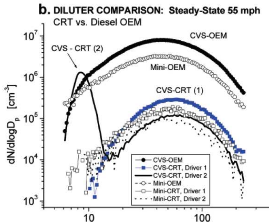
Figure 4. Comparisons of UFP number results using two different dilution methods – a constant volume sampler (“CVS-”) and a minidiluter (“Mini-”). The CVS method indicates higher UFP number with a CRT diesel engine that is not seen with the minidiluter technique (Holmén & Ayala, 2002).
