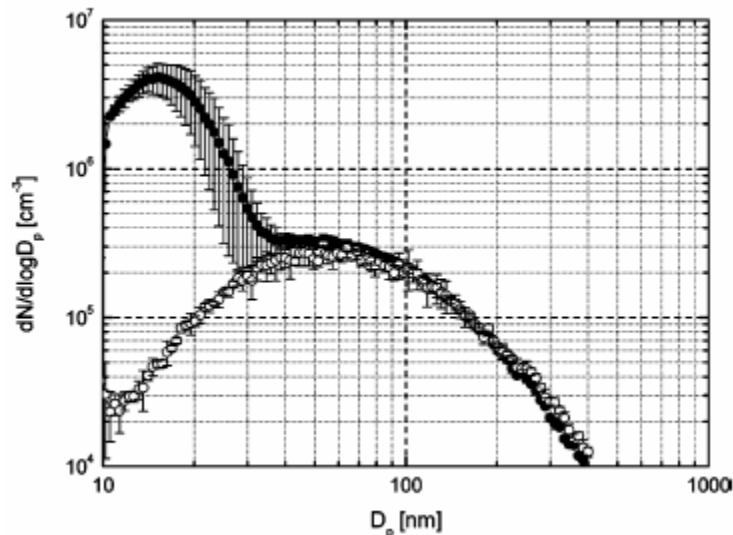
Figure 7. The size profile distribution shown in the figure indicates higher particle number below \sim 0.04 \mu\text{m} (40 nm) for low sulfur diesel (500 ppm S) (full circle profile) relative to the particle number for ultralow sulfur diesel (50 ppm S) (open circle profile) for a diesel engine with no control (Ristovski et al., 2006).
