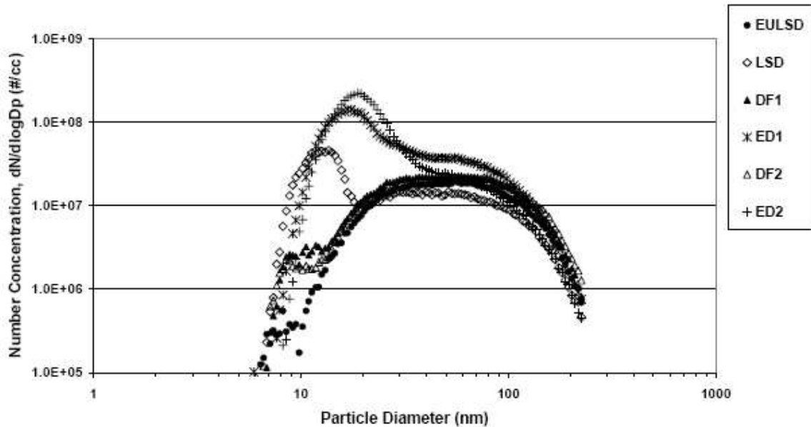
Figure 6. Profile of PM size distribution in diesel exhaust from an engine with no control. EULSD is <30 ppm sulfur; LSD is ~150 ppm sulfur; DF1 and DF2 are diesel with >400 ppm sulfur; ED1 and ED2 are 7 percent by volume ethanol blends with DF1 and DF2, respectively. The highest sulfur content diesel fuels (DF1 and DF2) and the ultralow diesel fuel (EULSD) display less bimodal character in the PM size distribution than the fuels with intermediate sulfur content (Frank et al., 2006).
