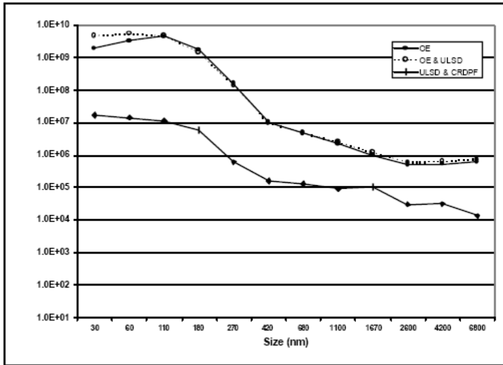
Figure 3. Particle number distributions in diesel engine exhaust from dynamometer test cycles. The figure shows the difference in PM number between an engine with no control (OE) run with and without <30 ppm sulfur diesel (ULSD) and a CRT diesel engine (CRDPF) with ULSD. The CRT results are from dynamometer testing of a bus after 12 months of on-road operation. The smallest PM size bin is \sim 0.03 \mu\text{m} (30 nm) (Chatterjee et al., 2002).
